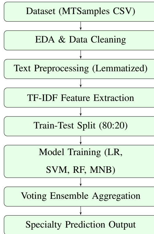
Figure 7: Activity Diagram of the Proposed Machine Learning Algorithm
